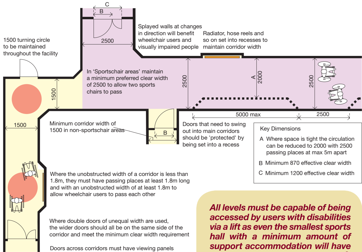
Note: All dimensions are in millimetres Internal circulation diagram
